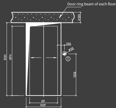
Landing door diagram
