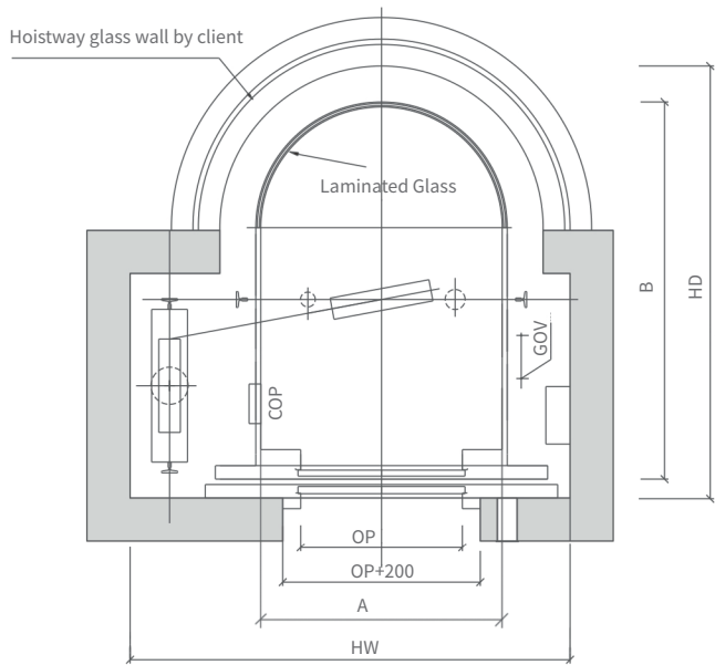
Hoistway Plan
