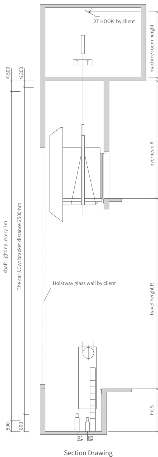
Section Drawing
